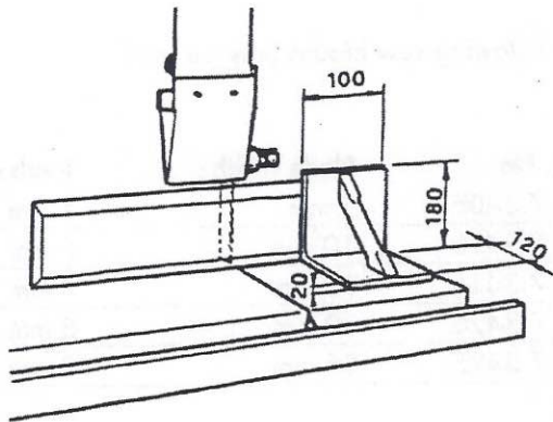
Fig. 7-9: Auxiliary fence
