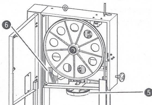
Fig. 7-3: Scale
