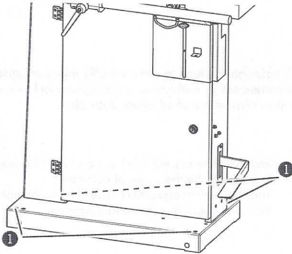
Fig. 6-1: Floor mounting
