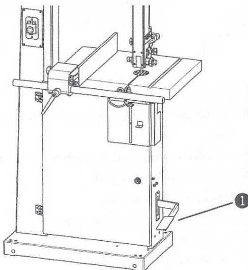
Fig. 5-3: Foot brake
