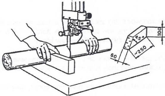
Fig. 7-8: Cutting a circular work-piece
