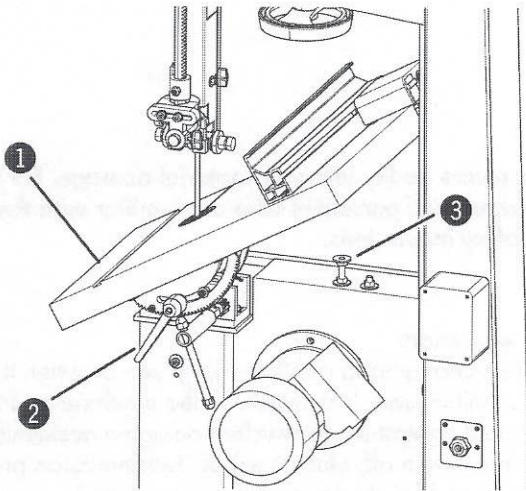
Fig. 6-3: End stop
