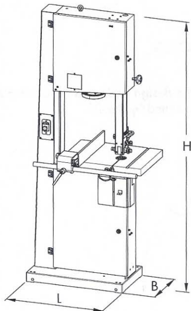
Fig. 4-1: Total size
