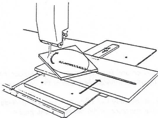
Fig. 7-12: Circular cuts
