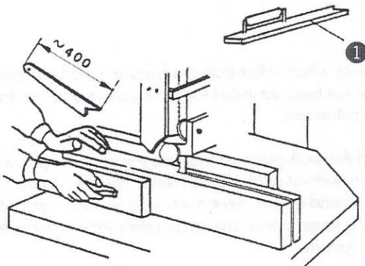
Fig. 7-10: Push stick
