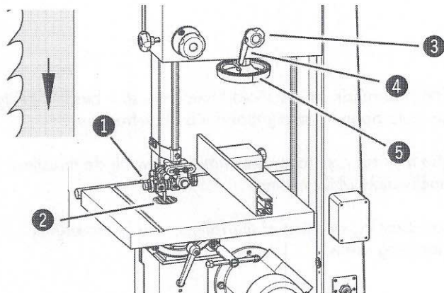
Fig. 7-2: Saw blade replacement
