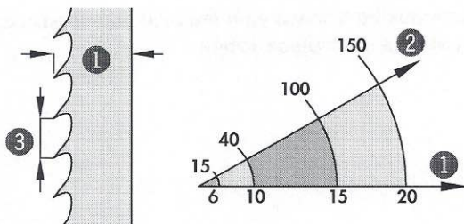
Fig. 7-6: Saw blades
